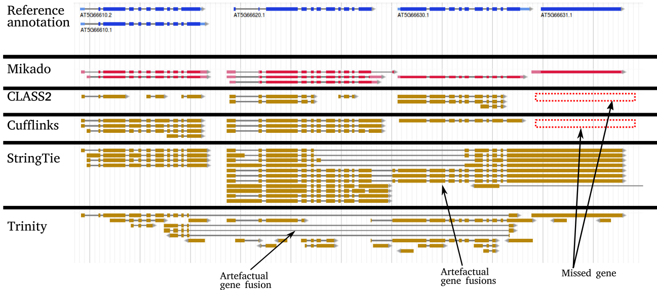
Figure 1: The algorithm employed by Mikado is capable of solving complex loci with multiple potential assemblies. This locus in A. thaliana is particularly challenging as an ancestral gene in the locus tandemly duplicated into the current AT5G66610, AT5G66620, and AT5G66630 genes. Due to these difficulties, no single assembler was capable of reconstructing all loci correctly. For instance, Trinity was the only method that correctly assembled AT5G66631, but it failed to reconstruct any other transcript correctly. The reverse was true for Cufflinks, which correctly assembled the three duplicated genes but completely missed the monoexonic AT5G66631. By choosing between different alternative assemblies, Mikado was capable to provide an evidence-based annotation congruent to the TAIR10 models.
