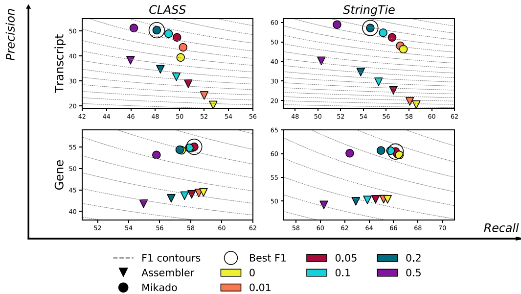
Figure 4: Performance of Mikado while varying the MIF parameter. Precision/recall plot at the gene and transcript levels for CLASS and StringTie at varying minimum isoform fraction thresholds in A. thaliana , with and without applying Mikado. Dashed lines mark the F1 levels at different precision and recall values. CLASS sets MIF to 5% by default (red), while StringTie uses a slightly more stringent default value of 10% (cyan).
