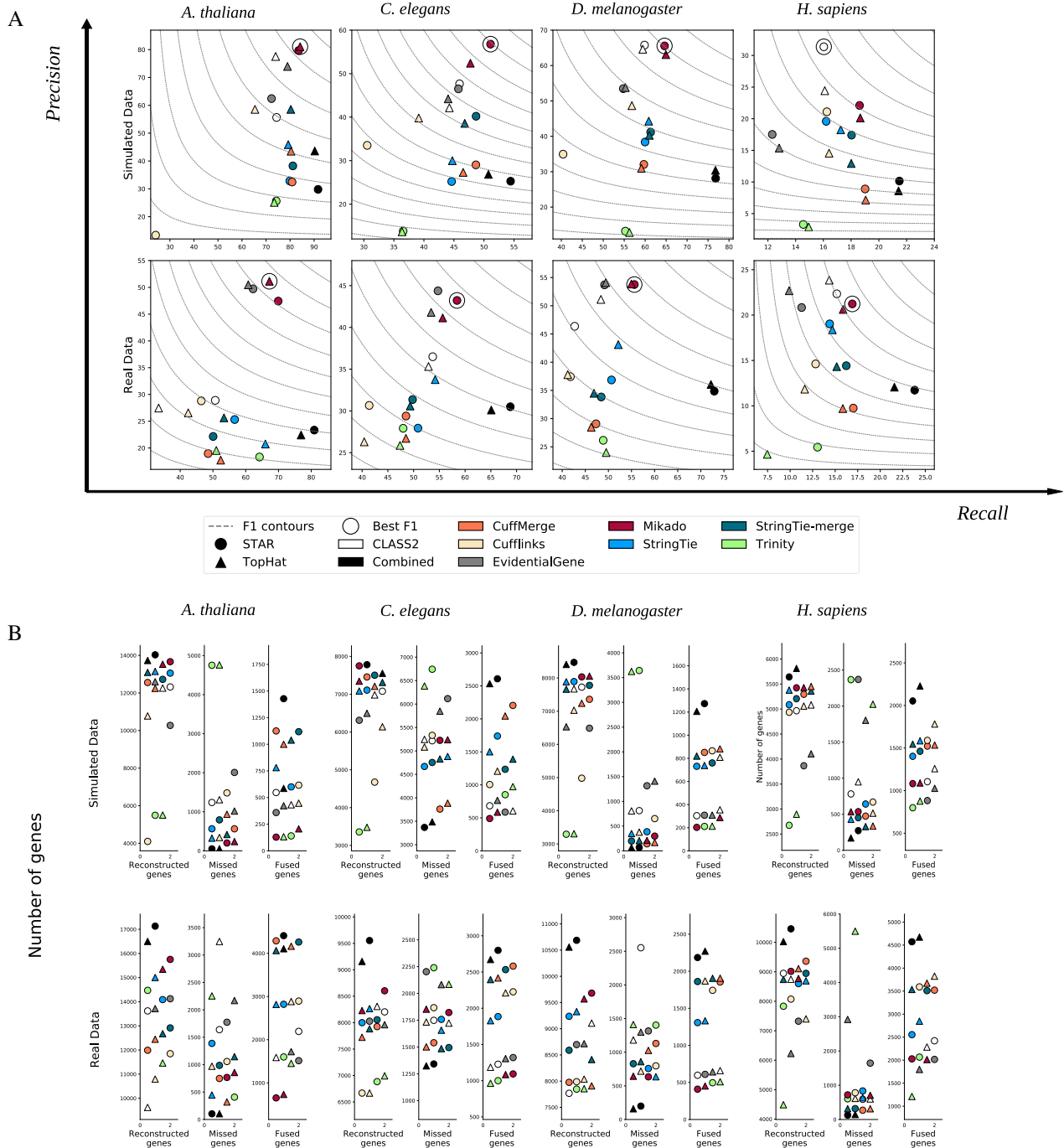
Figure 3: Performance of Mikado on simulated and real data. (A) We evaluated the performance of Mikado using both simulated data and the original real data. The method with the best transcript-level F1 is marked by a circle. (B) Number of reconstructed, missed, and chimeric genes in each assembly. Notice the lower level of chimeric events in simulated data.
