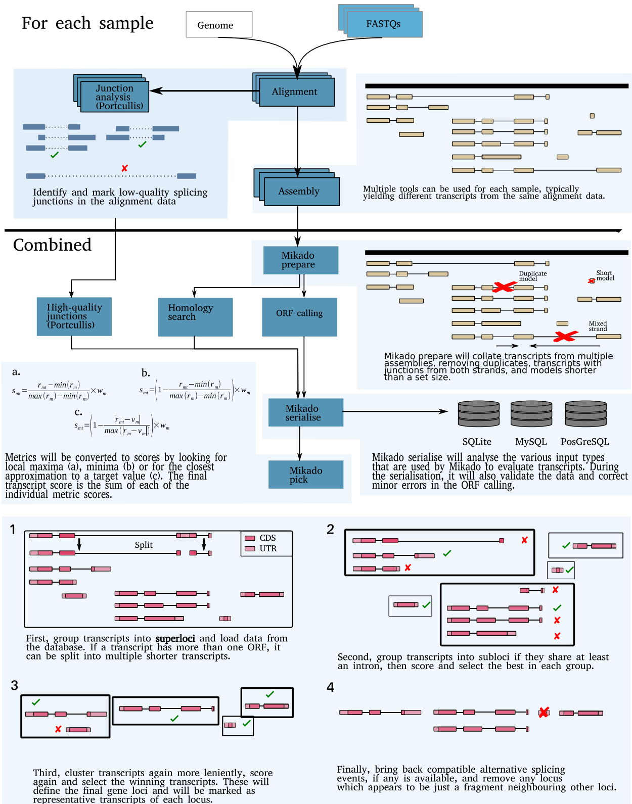
Figure 2: Schematic representation of the Mikado workflow.
